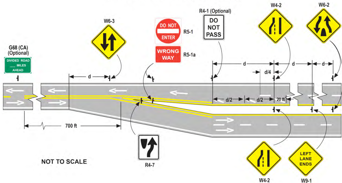
Figure 3B-14 (CA). Examples of Applications of Lane-Reduction Transition Markings (Sheet 2 of 3)
