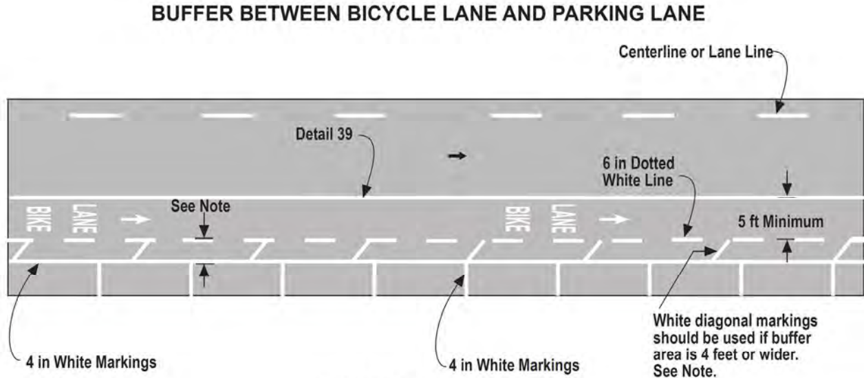
Figure 9C-104(CA). Examples of Markings for Buffered Bicycle Lanes Where Vehicle Parking is Prohibited/Permitted (Sheet 2 of 2)
