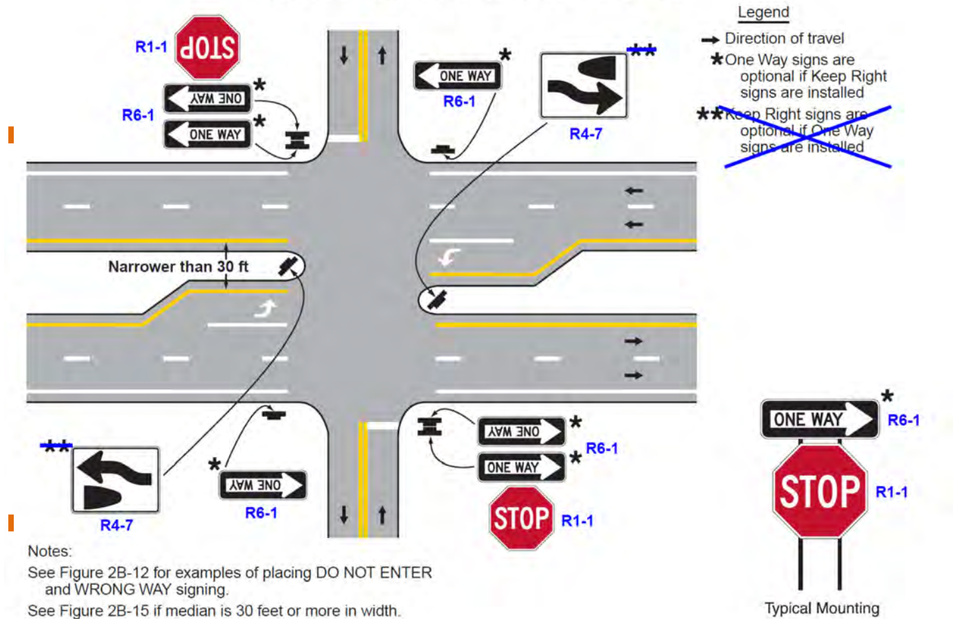
Figure 2B-16. ONE WAY Signing for Divided Highways with Median Widths Narrower Than 30 Feet
