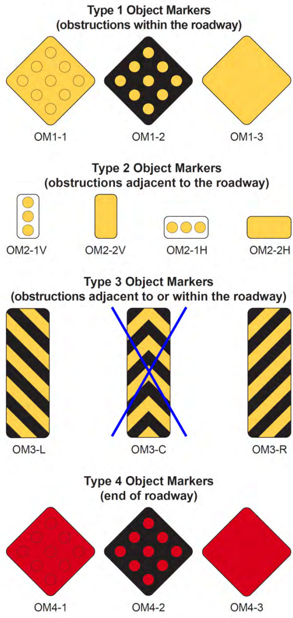
Figure 2C-13. Object Markers
