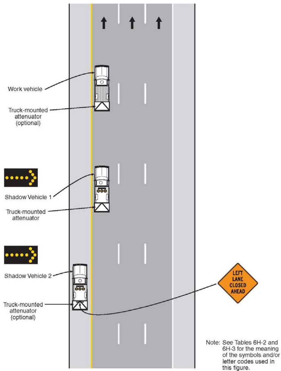
Typical Application 35
