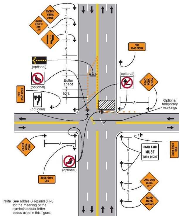
Typical Application 24
