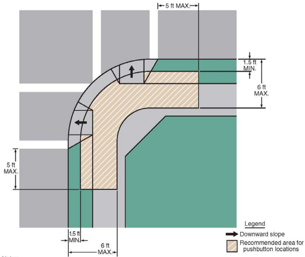
Figure 4E-3. Pushbutton Location Area
