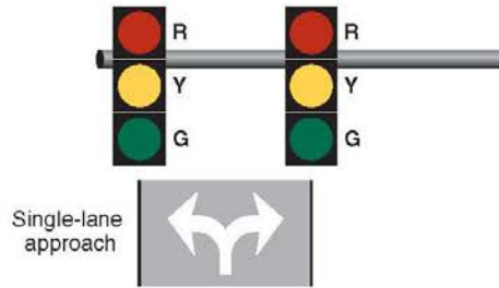
Figure 4D-20. Signal Indications for Approaches with a Shared Left-Turn/Right-Turn Lane and No Through Movement (Sheet 3 of 3)
