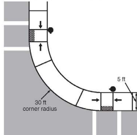
B - Parallel ramps with narrow sidewalk
