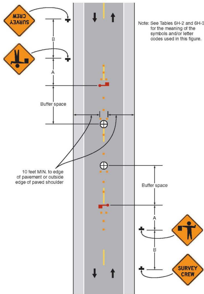
Typical Application 16
