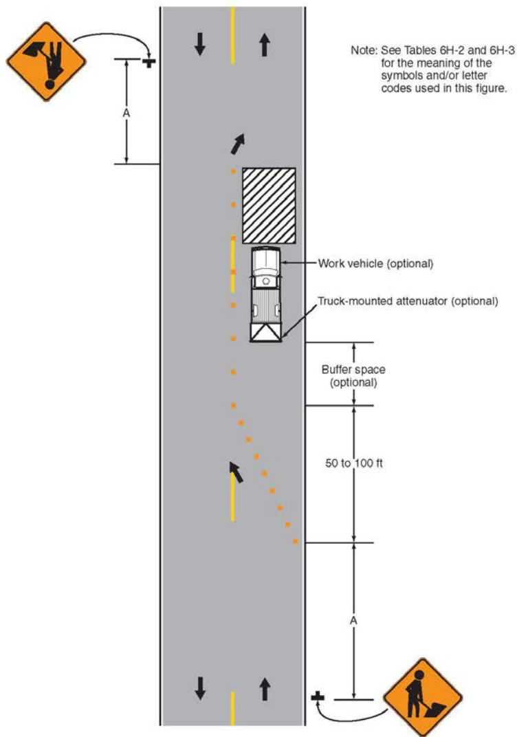
Typical Application 18
