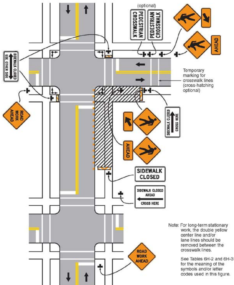
Typical Application 29
