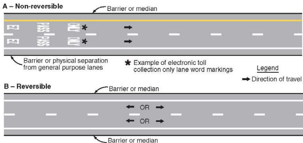
Figure 3D-1. Markings for Barrier-Separated Preferential Lanes
