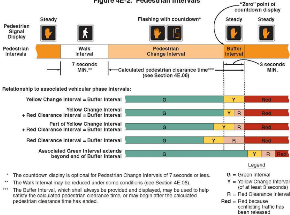
Figure 4E-2. Pedestrian Intervals
