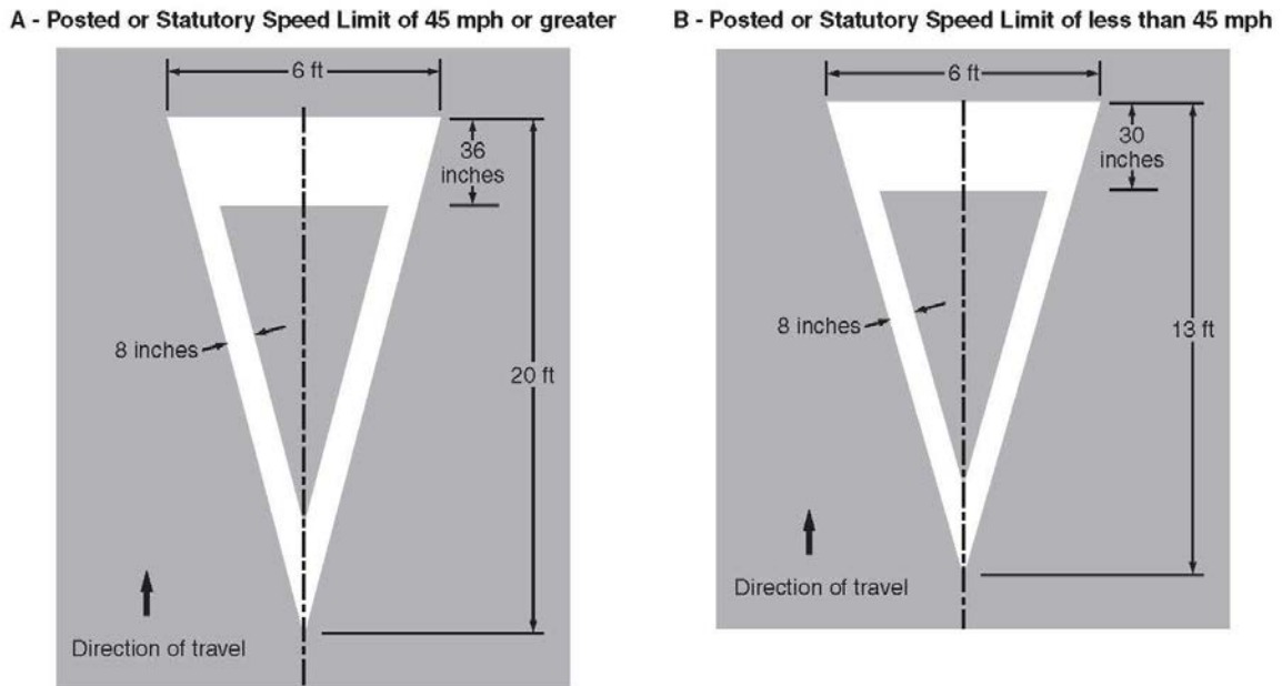
Figure 3B-26. Yield Ahead Triangle Symbols
