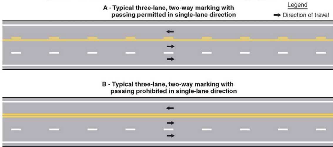
Figure 3B-3. Examples of Three-Lane, Two-Way Marking Applications
