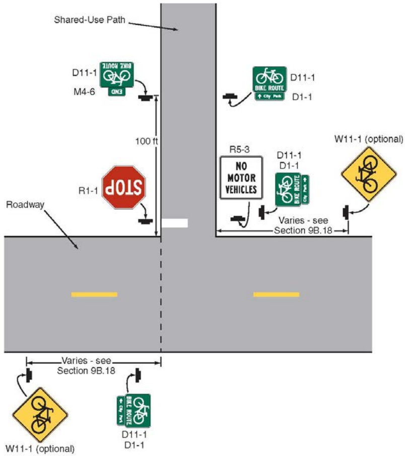
Figure 9B-6. Example of Bicycle Guide Signing
