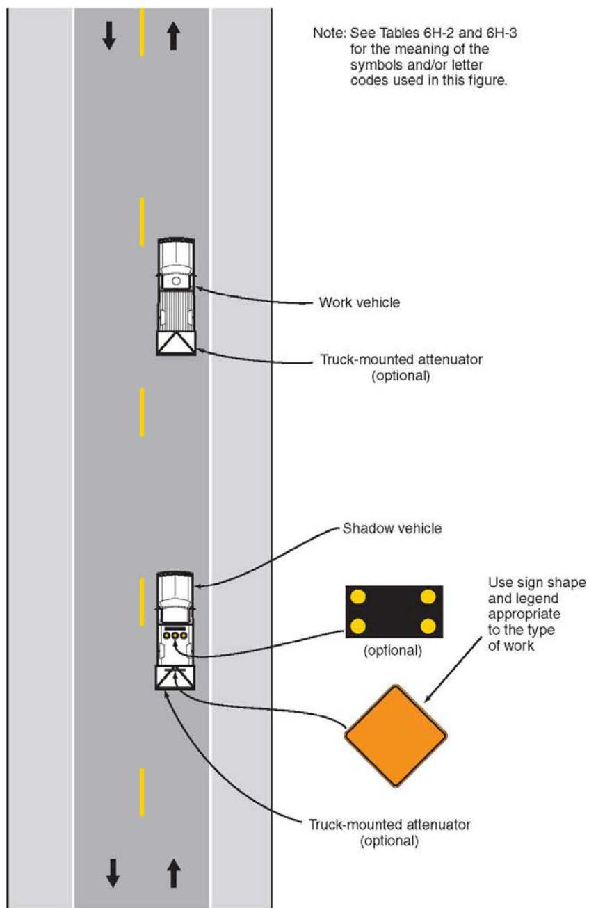
Typical Application 17
