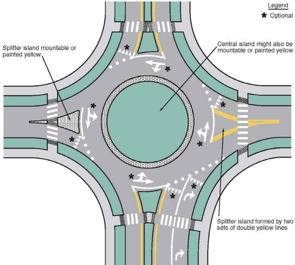
Figure 3C-3. Example of Markings for a One-Lane Roundabout
