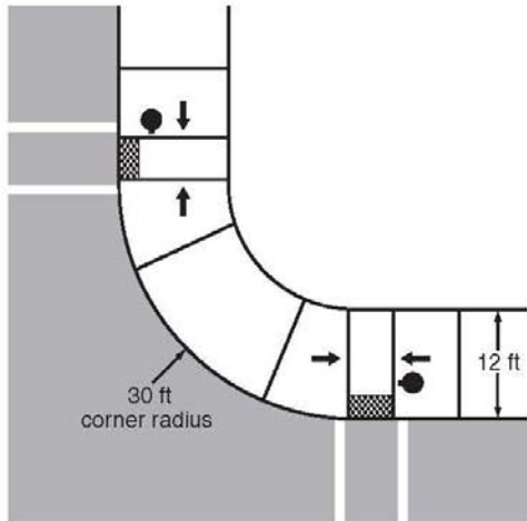
A - Parallel ramps with wide sidewalk
