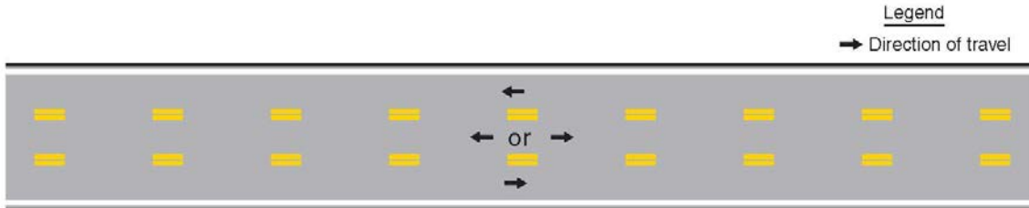
Figure 3B-6. Example of Reversible Lane Marking Application
