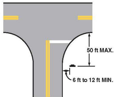
F - WIDE THROAT INTERSECTION
