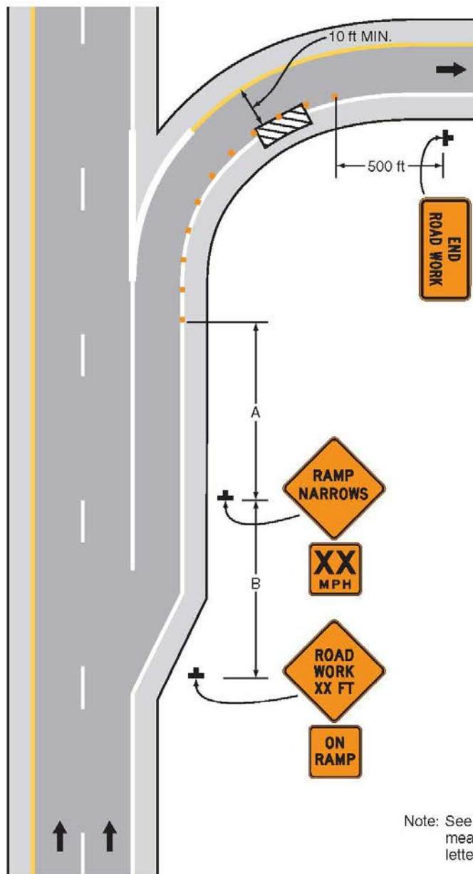
Typical Application 43
