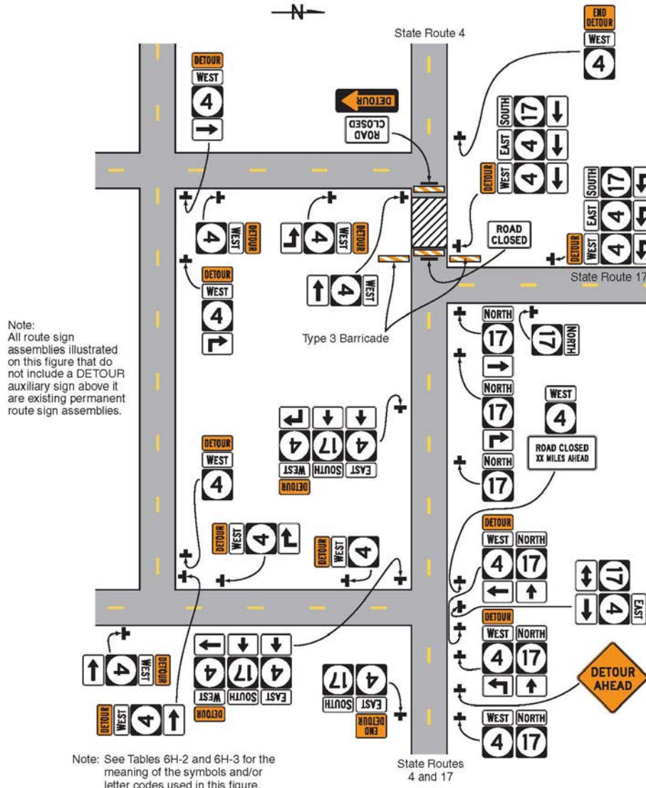
Typical Application 9
