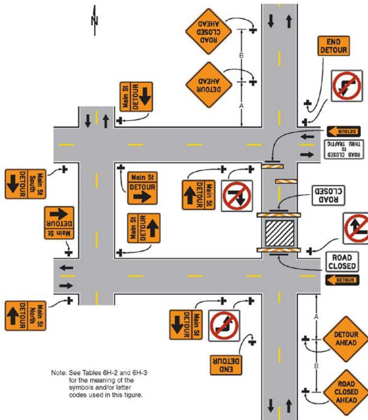
Typical Application 20
