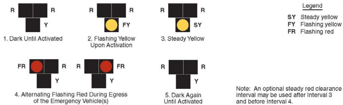
Figure 4G-1. Sequence for an Emergency-Vehicle Hybrid Beacon
