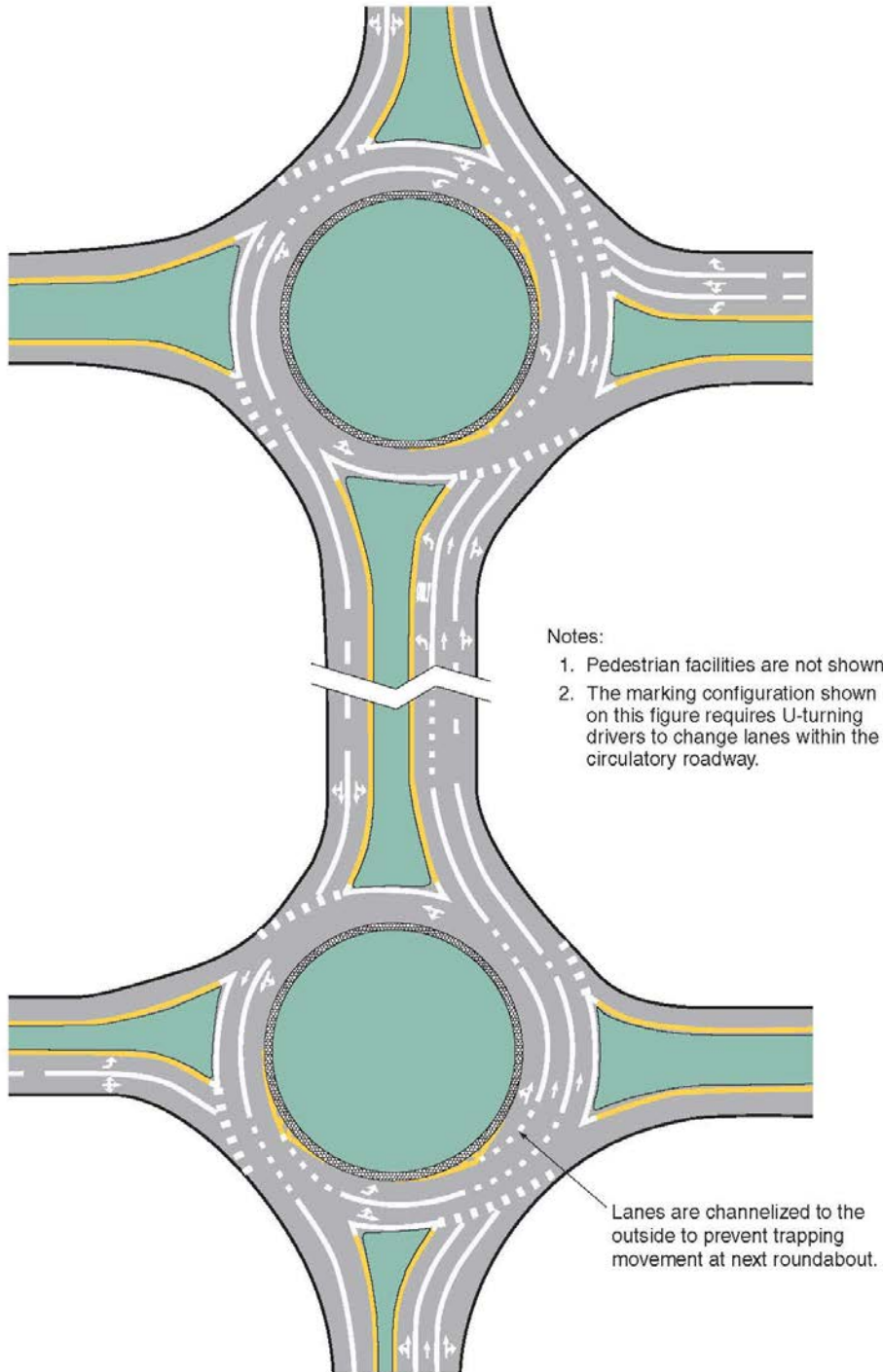
Figure 3C-13. Example of Markings for Two Linked Roundabouts
