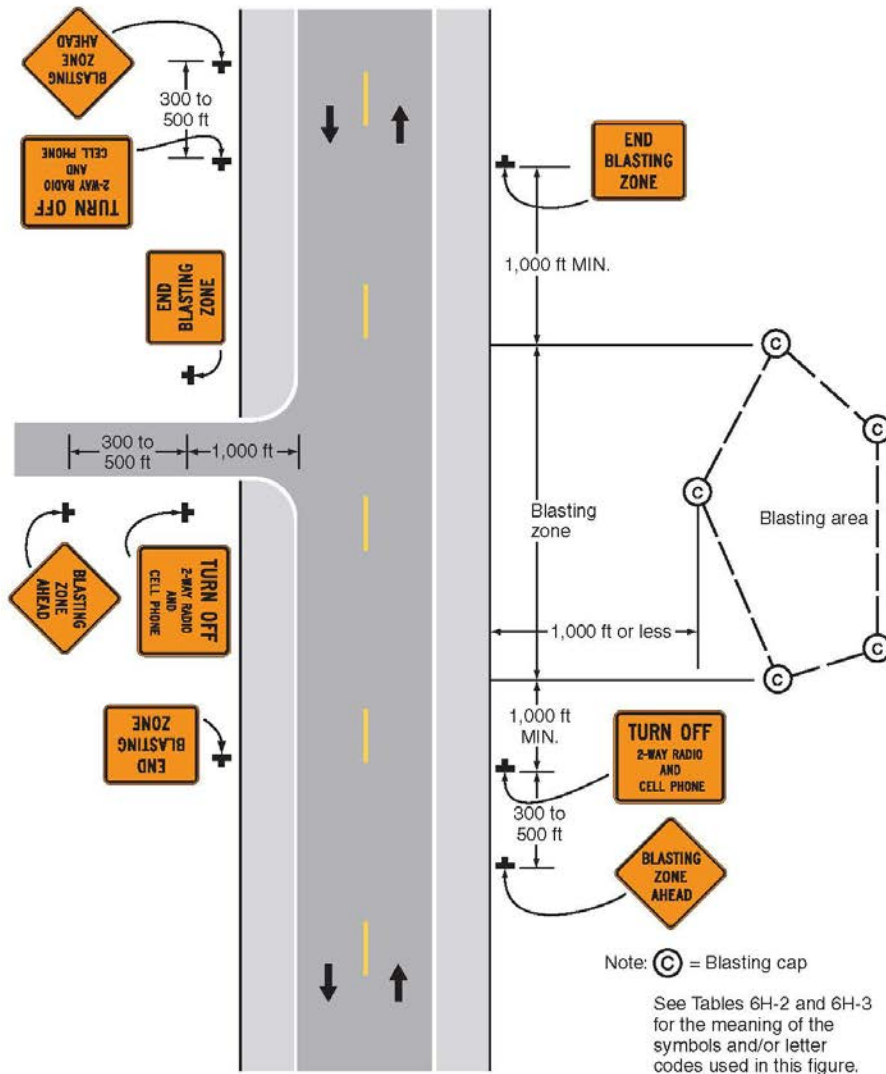
Typical Application 2
