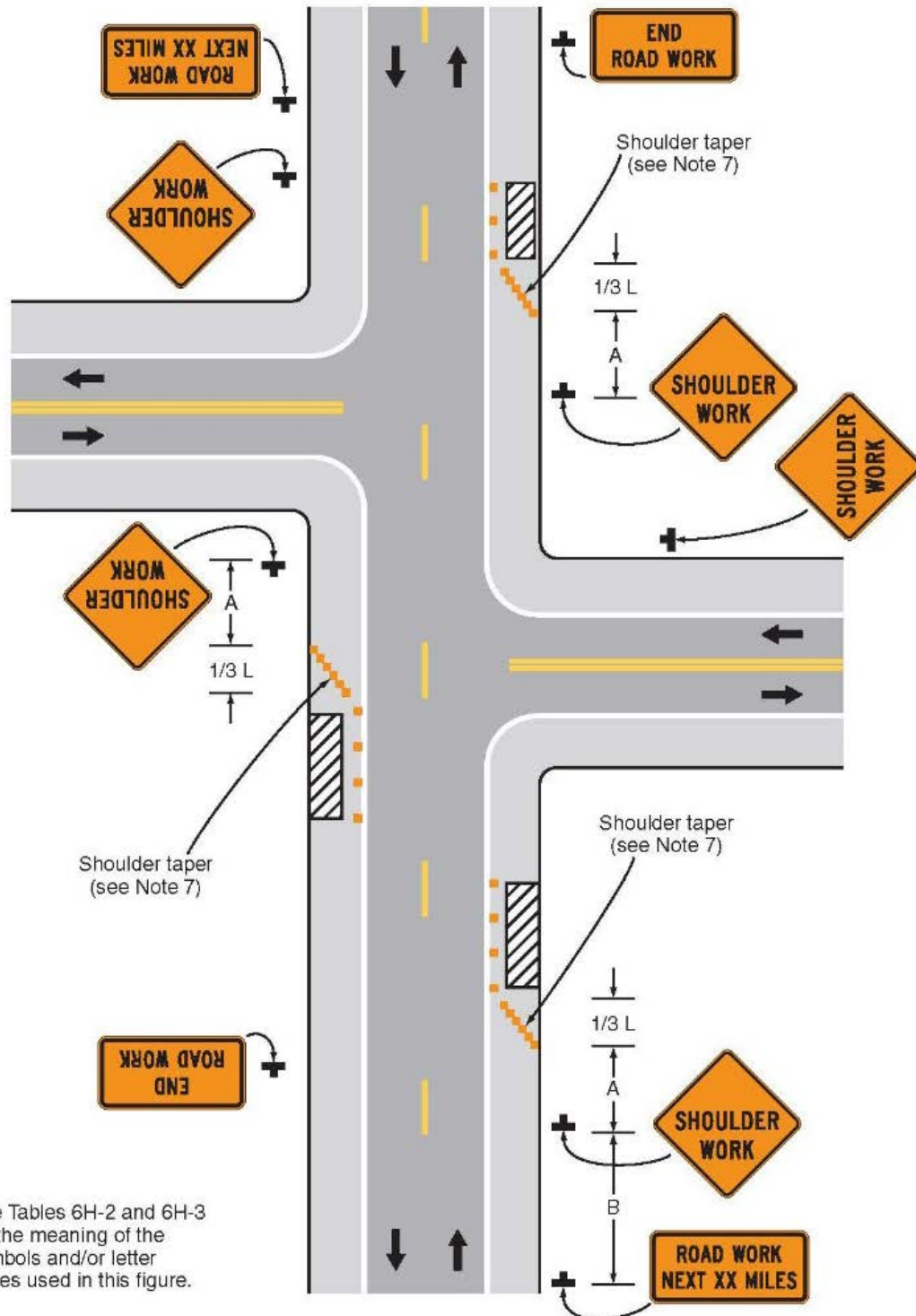
Typical Application 3
