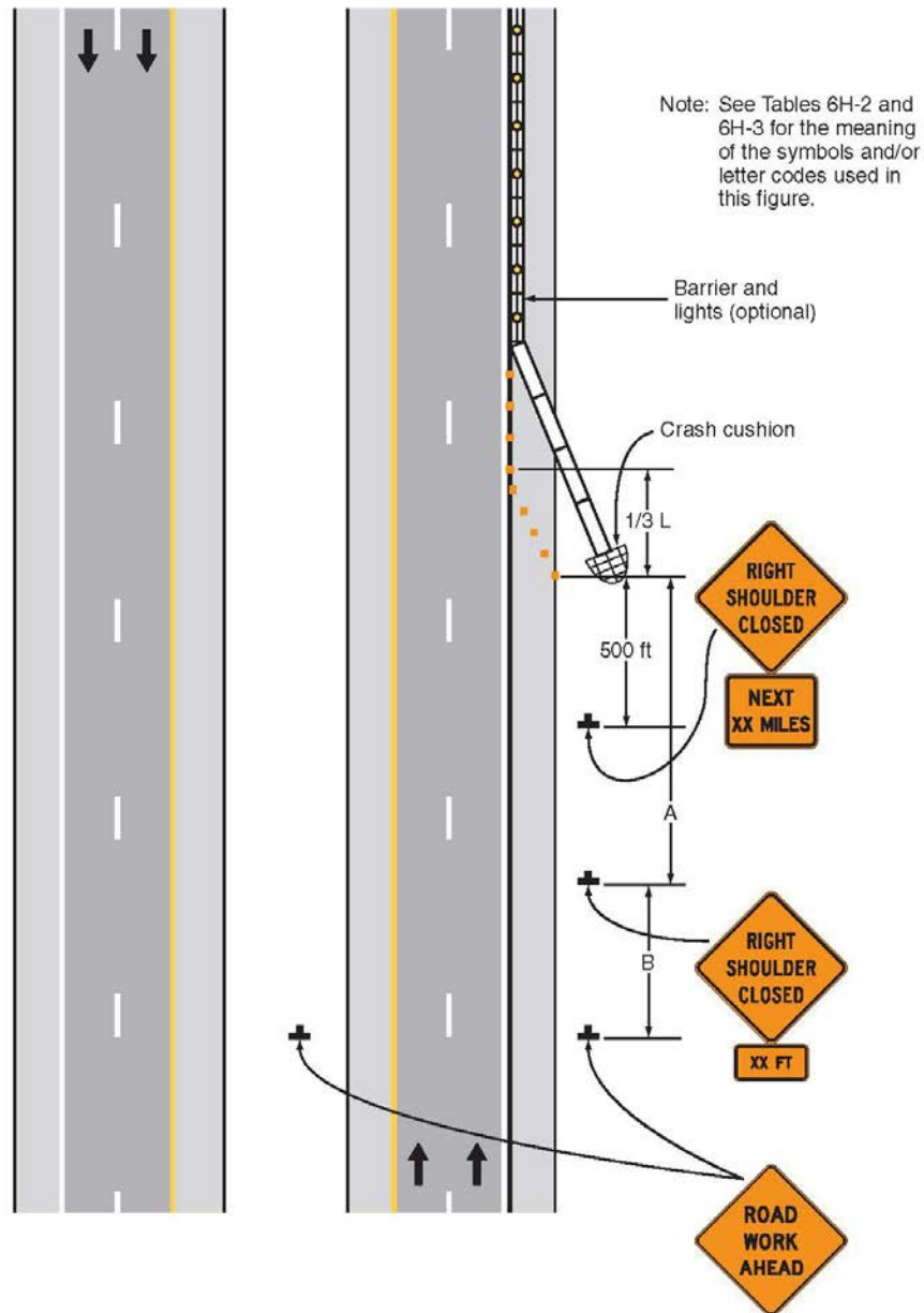
Typical Application 5
