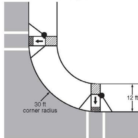
D - Perpendicular ramps with crosswalks far apart
