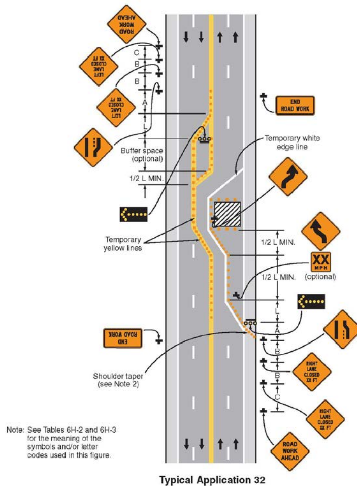
Figure 6H-32. Half Road Closure on a Multi-Lane, High-Speed Highway (TA-32)
