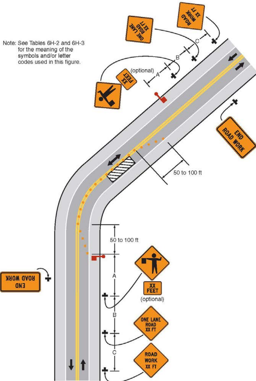
Typical Application 10
