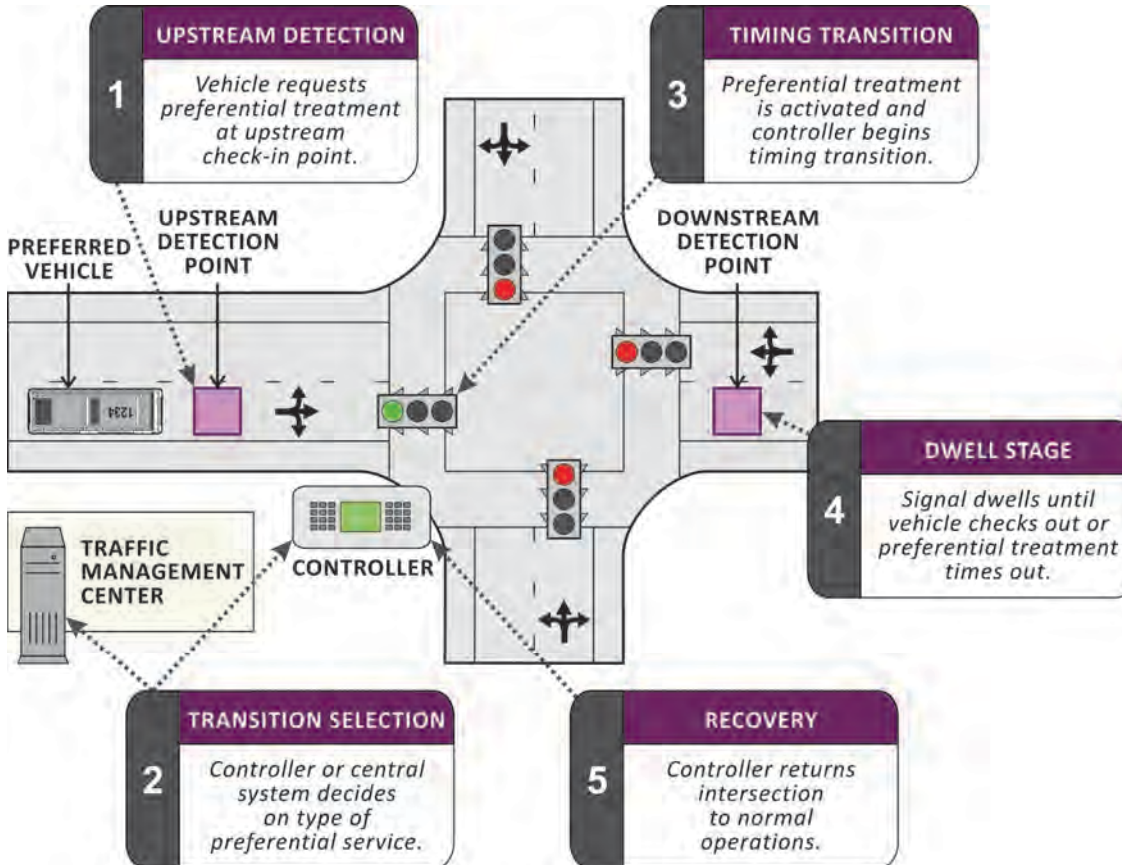
Exhibit 10-2 Preferential Treatment Process
