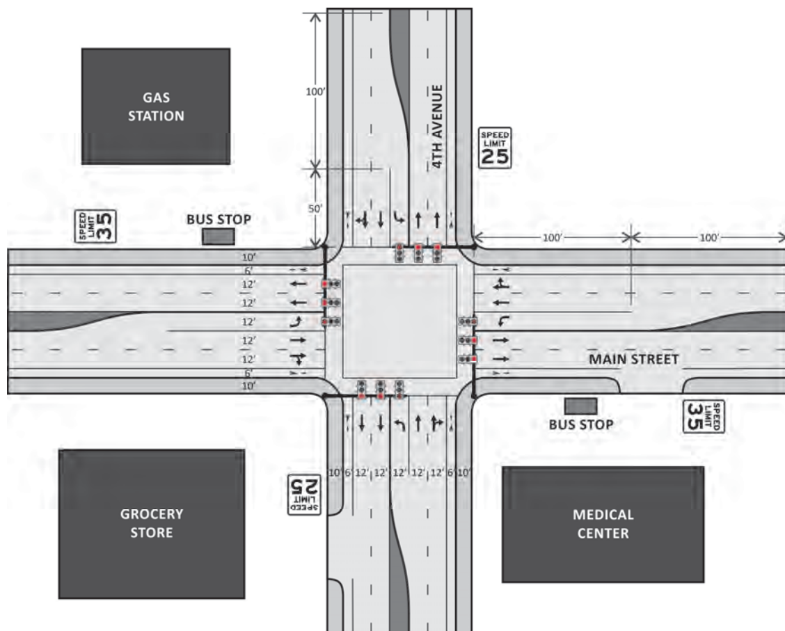
Exhibit 3-15 Example Intersection Condition Diagram
