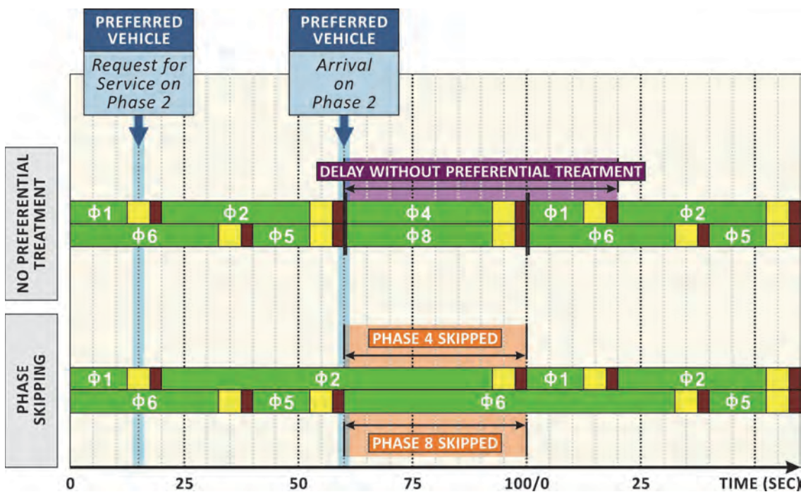
Exhibit 10-9 Phase Skipping
