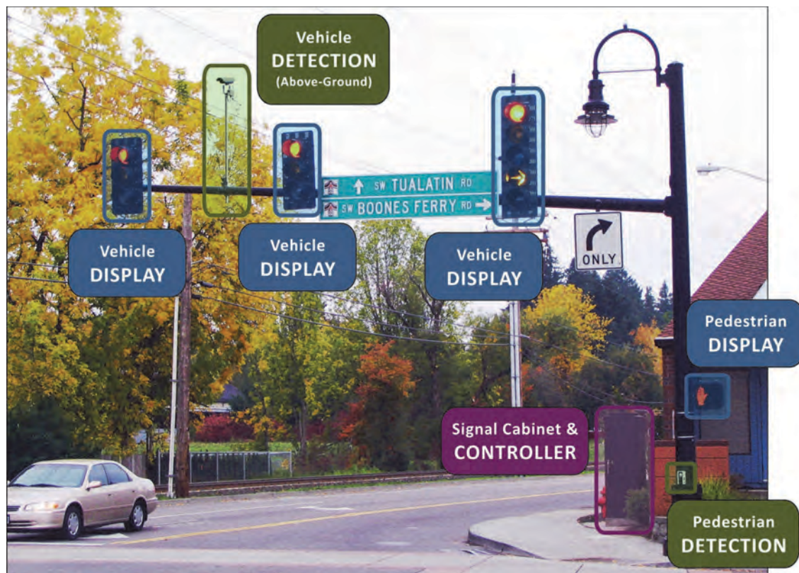
Exhibit 3-2 Common Signalized Intersection Components
