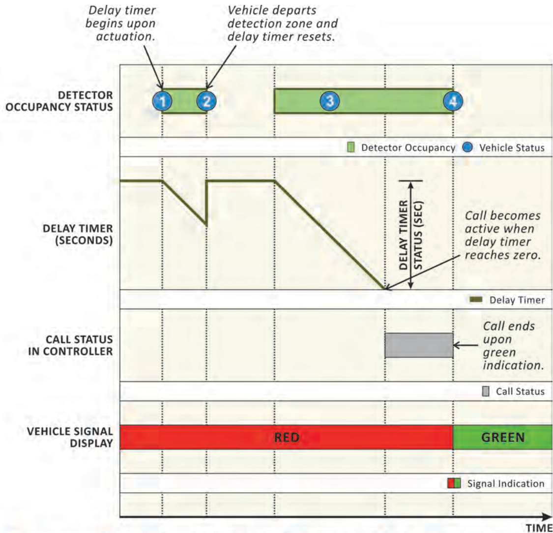
Exhibit 6-23 Delay Timer
