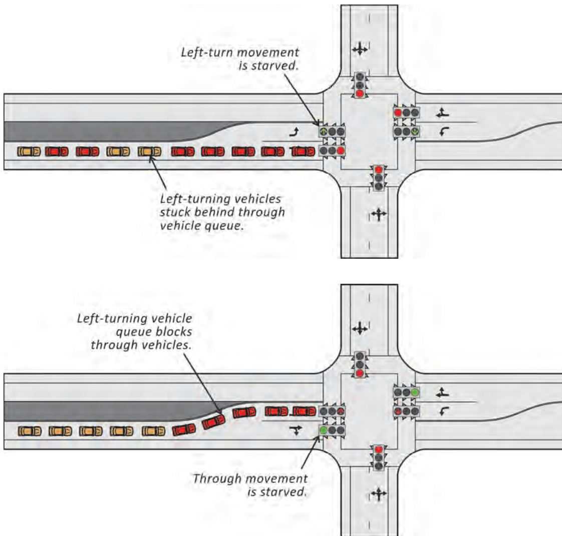
Exhibit 3-21 Storage Bay Blocking
