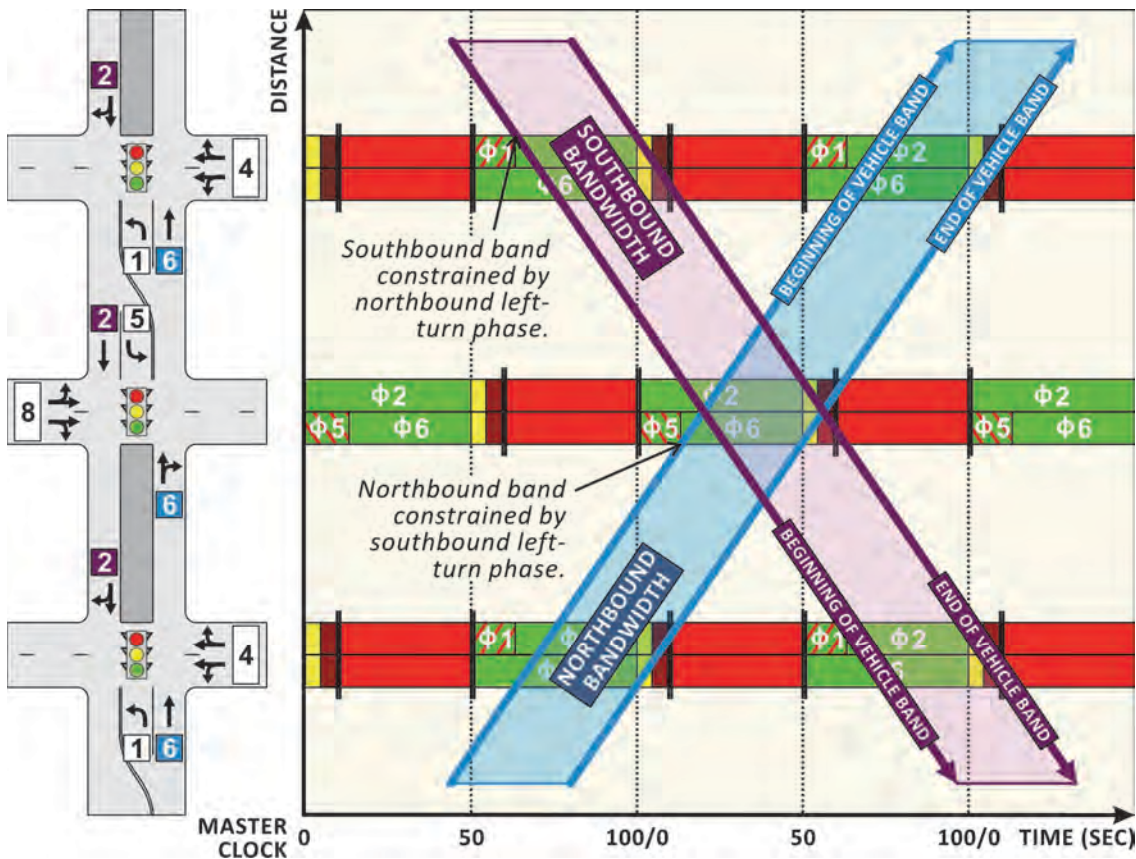
Exhibit 7-8 Bandwidth
