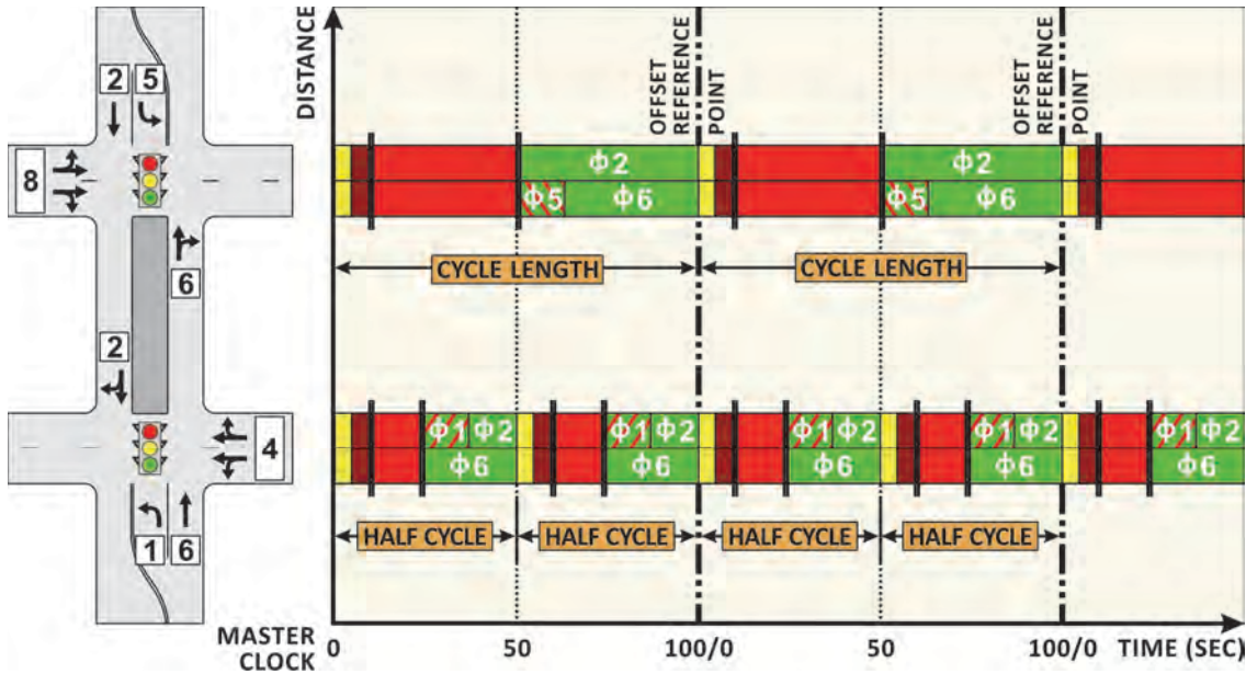
Exhibit 7-11 Cycle Length
