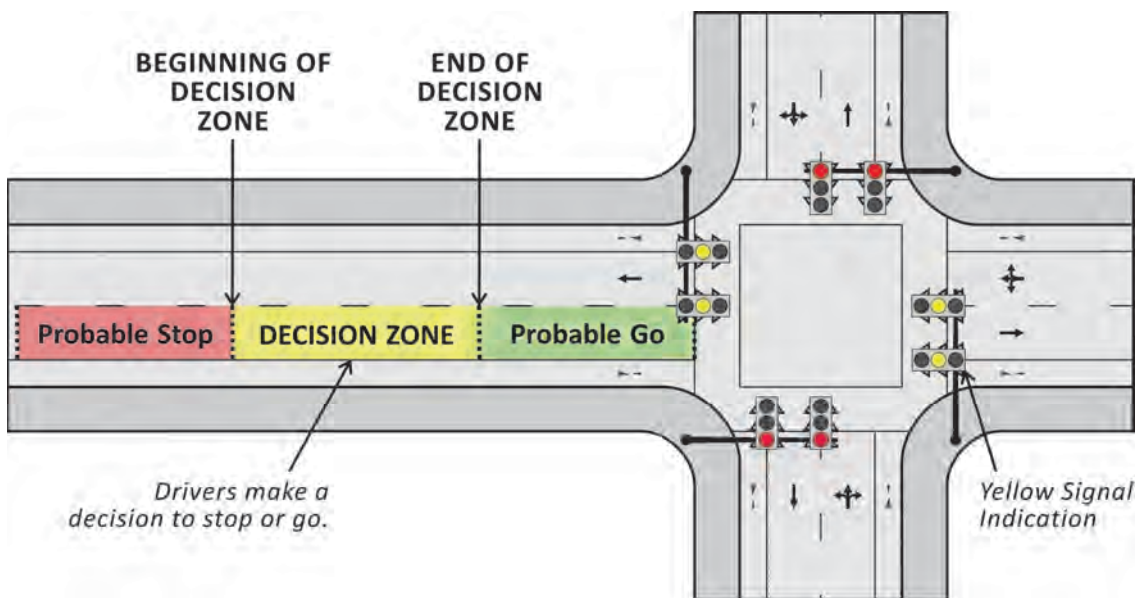
Exhibit 4-6 Decision Zone
