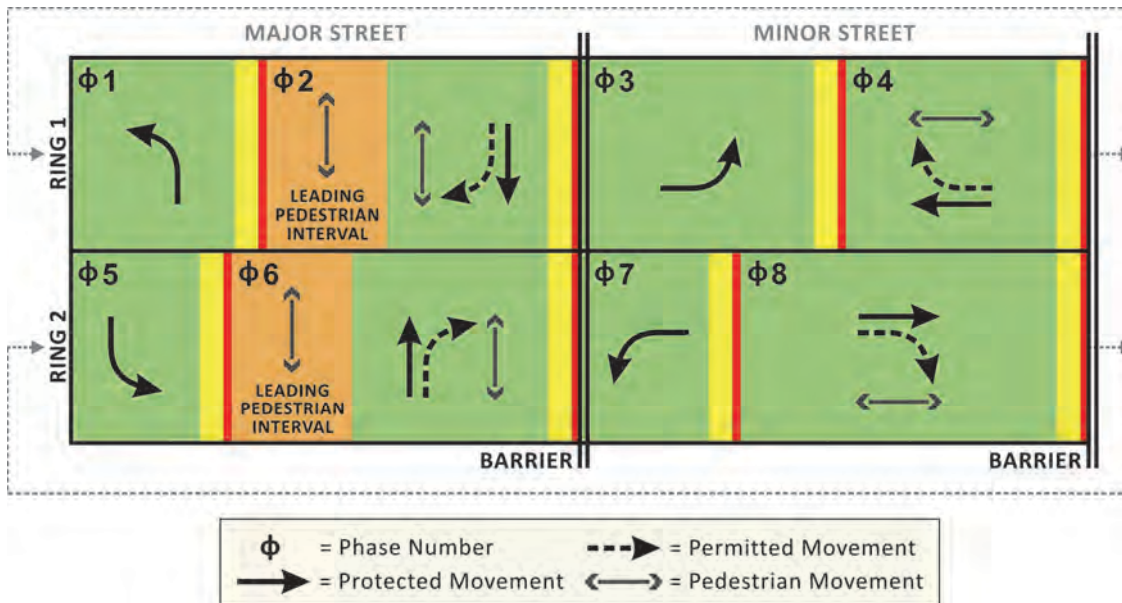
Exhibit 6-20 Leading Pedestrian Intervals
